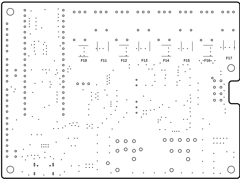
View from Bottom side (Scale 1:1)
